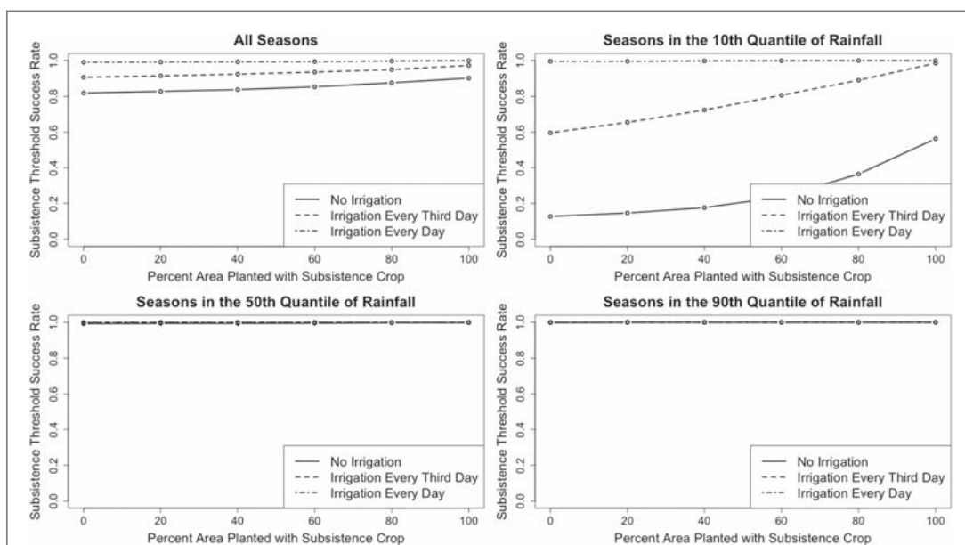
Figure 1. Fraction of growing seasons exceeding the minimum subsistence threshold plotted against the percent area planted with subsistence crop for the simulation average and selected quantiles.
