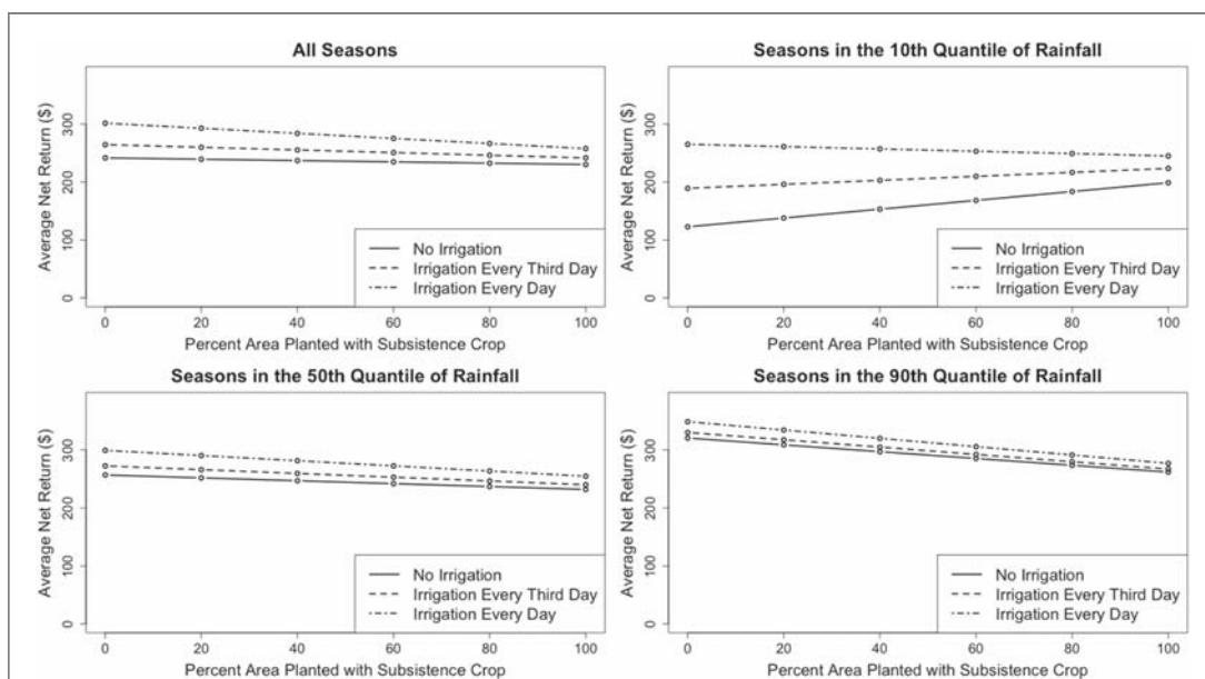
Figure 2. Average net return plotted against the percent area planted with subsistence crop for the simulation average and selected quantiles.
