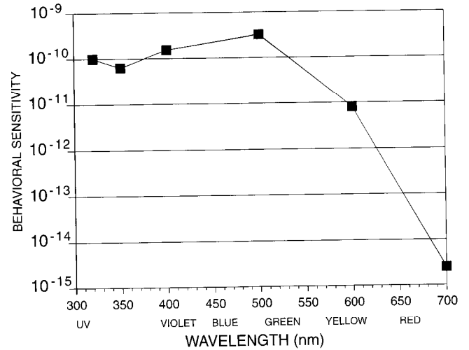
Figure 6. Behavioral sensitivity of loggerhead hatchlings to low-intensity colored light, represented as the inverse of the light-source radiance required to evoke significantly directed orientation in groups of hatchlings ( n = 30 per wavelength). At the low light levels represented here (approximately the radiance of the sky on a full-moon night, and dimmer), there was orientation toward the light source at all wavelengths. The ordinate is a log scale of the units (photons/s/m 2 /sr) -1 . Data are from Witherington (1992b). Figure adapted from Witherington (in press) and Lohmann et al. (in press); used with permission.
