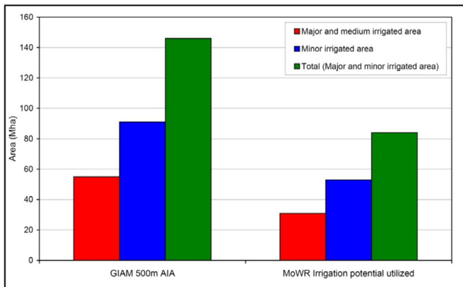
Figure 5. GIAM 500-m annualized irrigated areas (AIA) for India versus India’s Ministry of Water Resources (MoWR) derived irrigation potential utilized (IPU).
