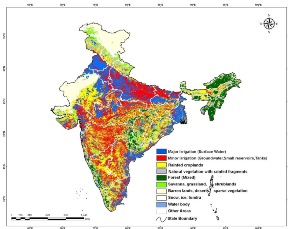
Figure 11. The irrigated plus rain-fed cropland areas of India along with other land-use/land-cover (LULC) classes from the GIAM 10 km. Of the 330 Mha of geographic area, 101 Mha are irrigated, 49 Mha rain-fed and the rest other LULC.
