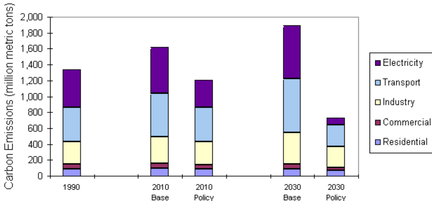
FIG. 3. Carbon emissions from fossil fuel combustion for the base case (Base) and the innovation path (Policy).
