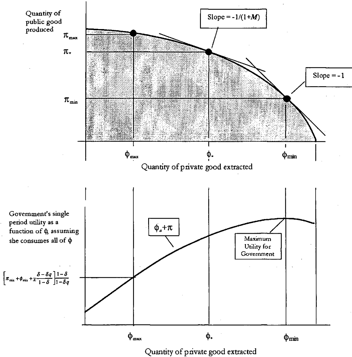
Figure 2: Production Possibility Set and Graphical Representation of \pi_{\min} , \pi_* and \pi_{\max} .
