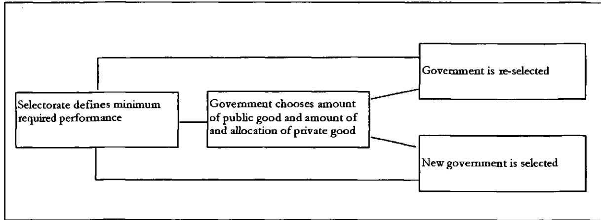
Figure 1: Game Tree
