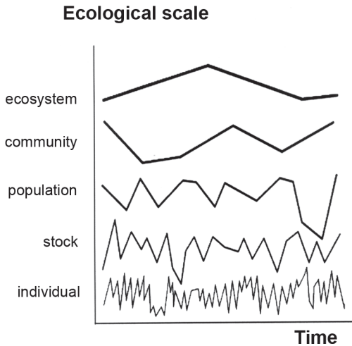
Figure 1: The relative time-steps (rate of variation) at the different scales of an ecosystem. (Sketched from O'Neill, et al., 1986 and Allen and Hoekstra, 1992.)
