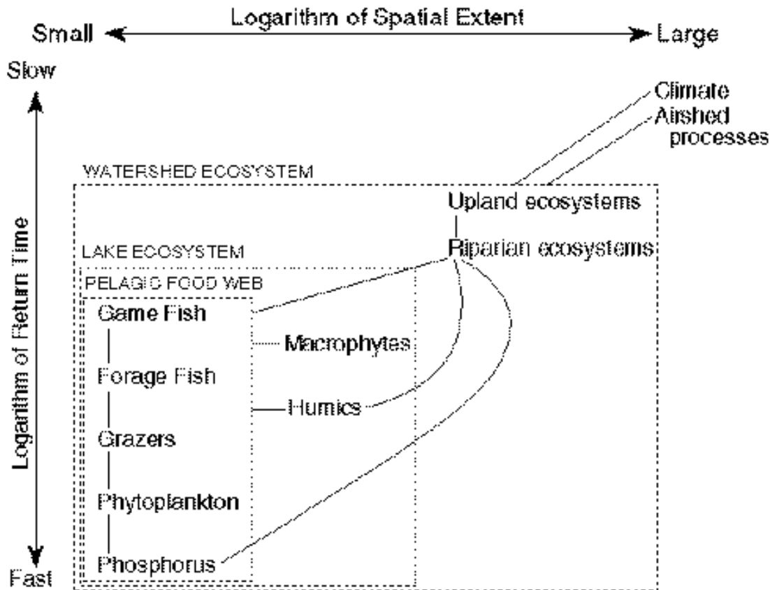
Fig. 1. Major interactions in the normal dynamics of lakes as a function of spatial extent (x-axis) and return time (y-axis). Boxes enclose 3 commonly-recognized subsystems: the watershed (largest box), lake (medium-size box), and pelagic zone (smallest box).
