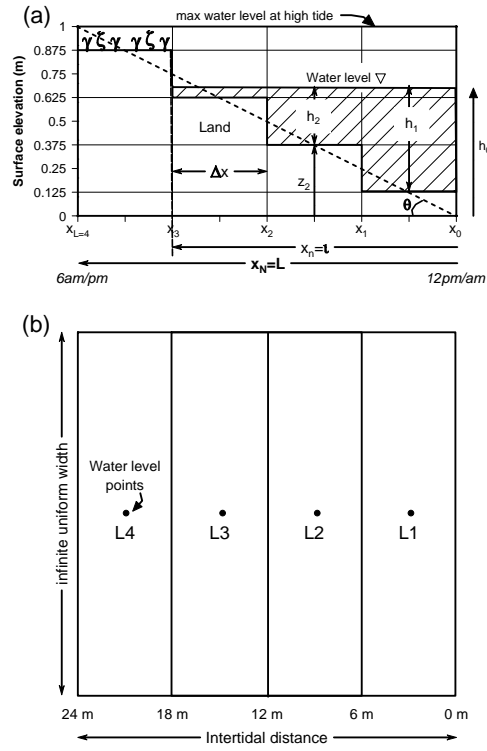
Fig. 2. Conceptual model for tidal wetland geometry: (a) Profile view: Elevation and profile length of terraces correspond to mean wetland bed slope \theta , and schematic vegetation shown only on upper terrace for clarity; (b) Plan view.
